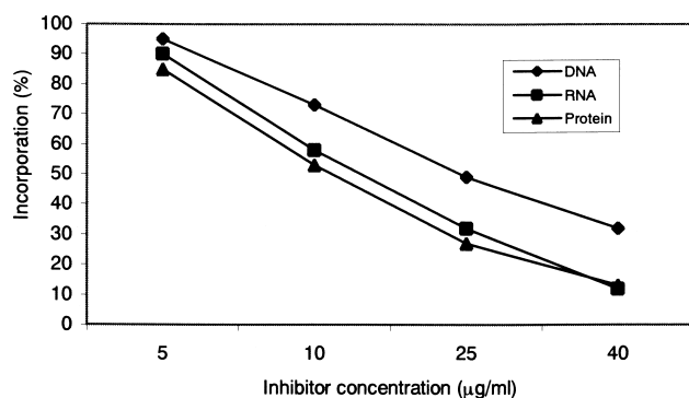
Fig. 2 Inhibitory effect of favolon B on incorporation of radio-labelled precursors into macromolecules HL-60 cells. [ ^{14}\text{C} ] thymidine into DNA, control 61267 cpm; [ ^{14}\text{C} ] uridine into RNA, control 124829 cpm; [ ^{14}\text{C} ] leucine into proteins, control 18837 cpm.
