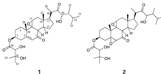
Fig. 1 Relative structures of favolon B ( 1 ) and favolon ( 2 ).
